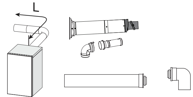
Horizontal flue with 90° elbow(s)
